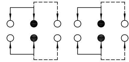
SCHEMATIC (NON-SHORTING)
